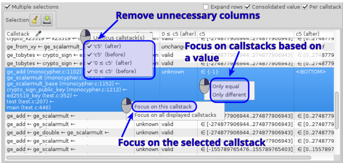
Figure 4.6: Callstacks display
