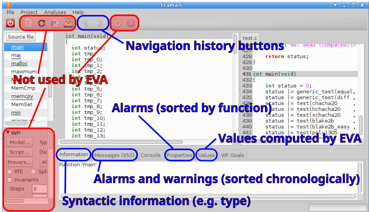
Figure 4.1: Frama-C GUI for Eva
