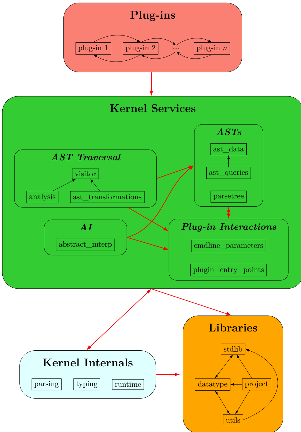
Figure 3.1: Frama-C Architecture Design.
