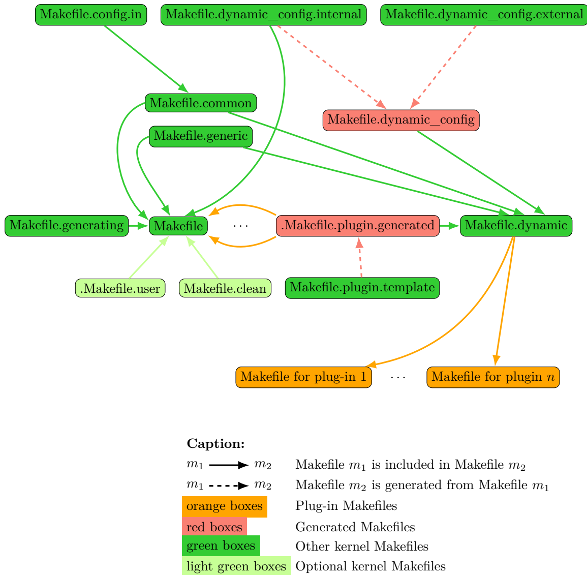
Figure 5.2: Relationship between the Makefiles
