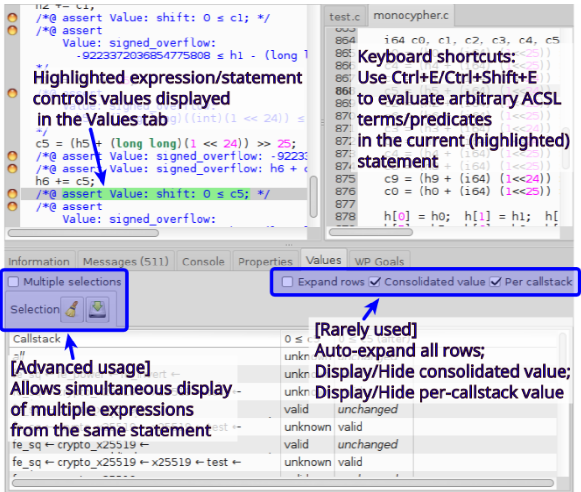
Figure 4.4: Values panel
