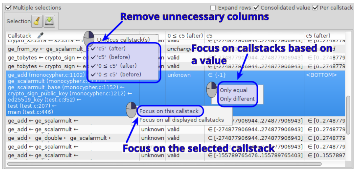
Figure 4.6: Callstacks display
