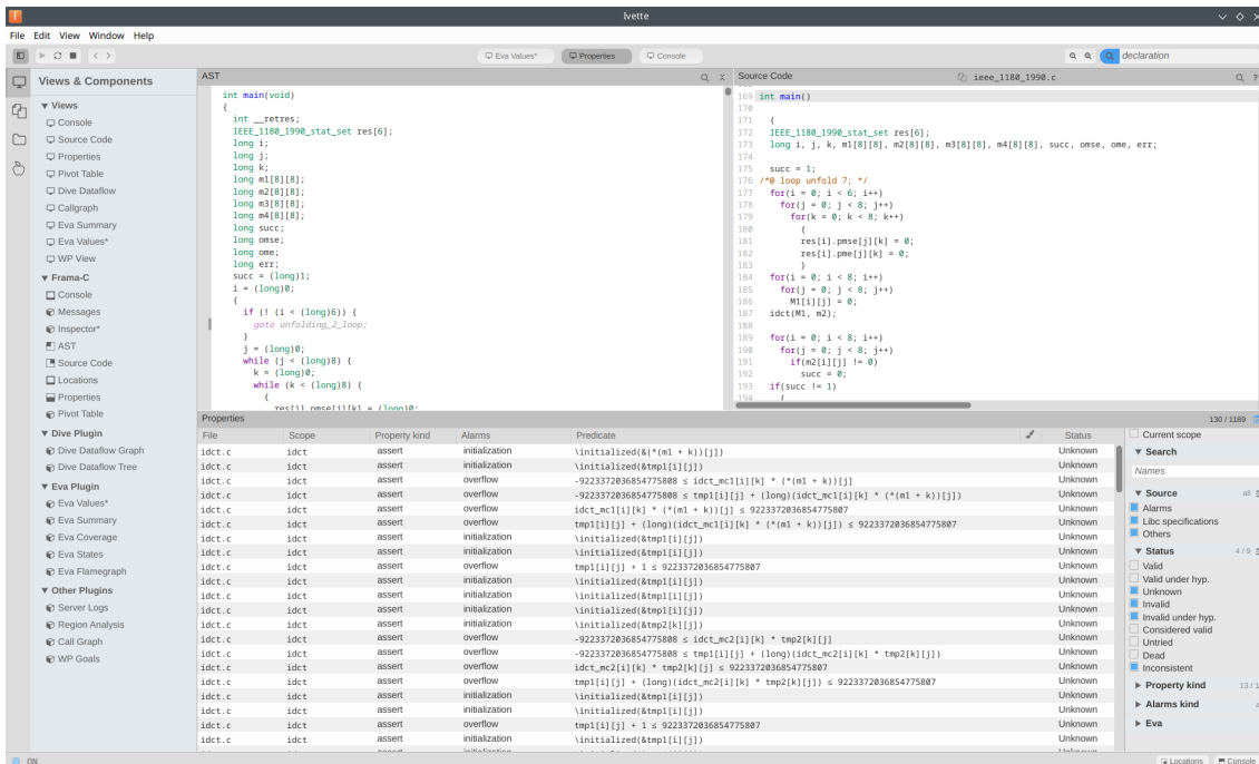
Figure 10.1: Screenshot of Ivette, illustrating several components
