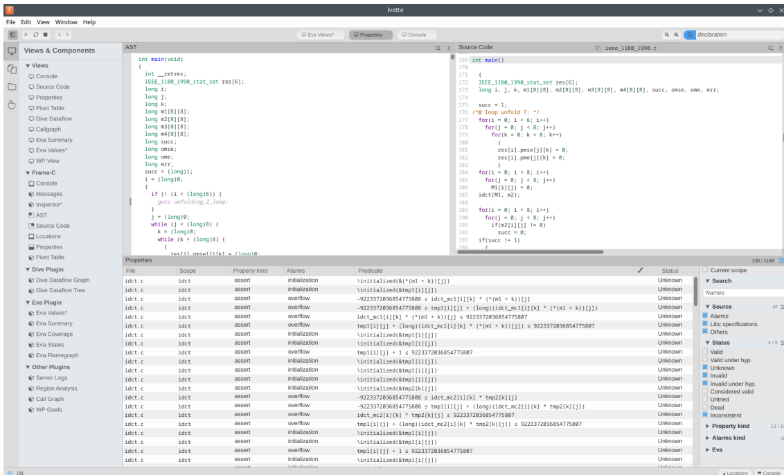
Figure 10.1: Screenshot of Ivette, illustrating several components
