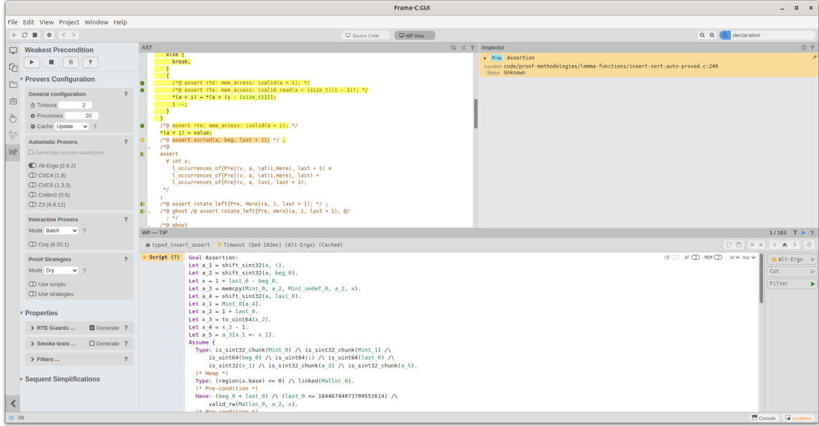
Figure 2.4: Interactive Proof Editing
